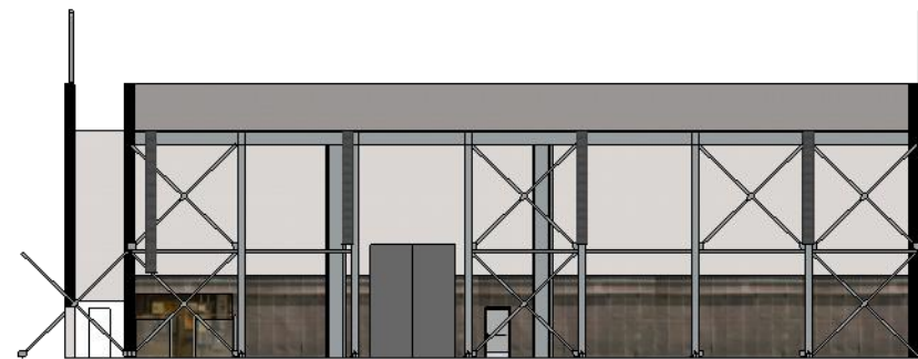
N ELEV NORTH scale: 1" = 30' [1:360]
