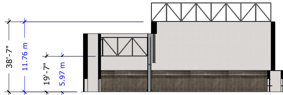
E ELEV EAST scale: 1" = 30' [1:360]
