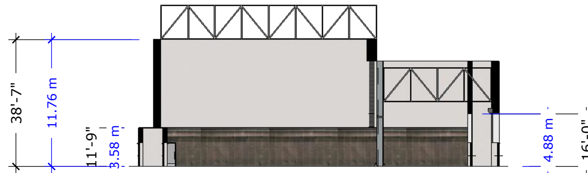
W ELEV WEST scale: 1" = 30' [1:360]
